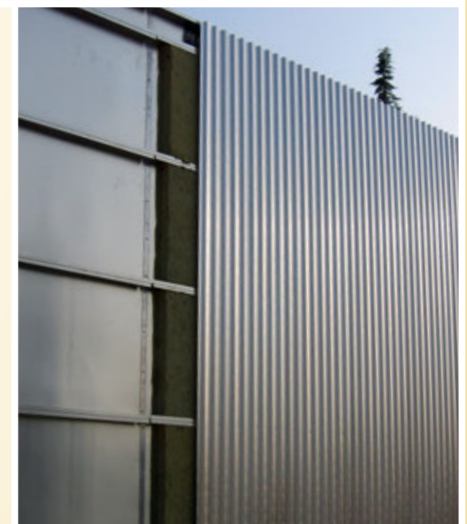
Copertura Cassetti e Lana Minerale con Lamiere Greccate Drawers and Mineral Wool cover with corrugated sheets Внешнее покрытие
